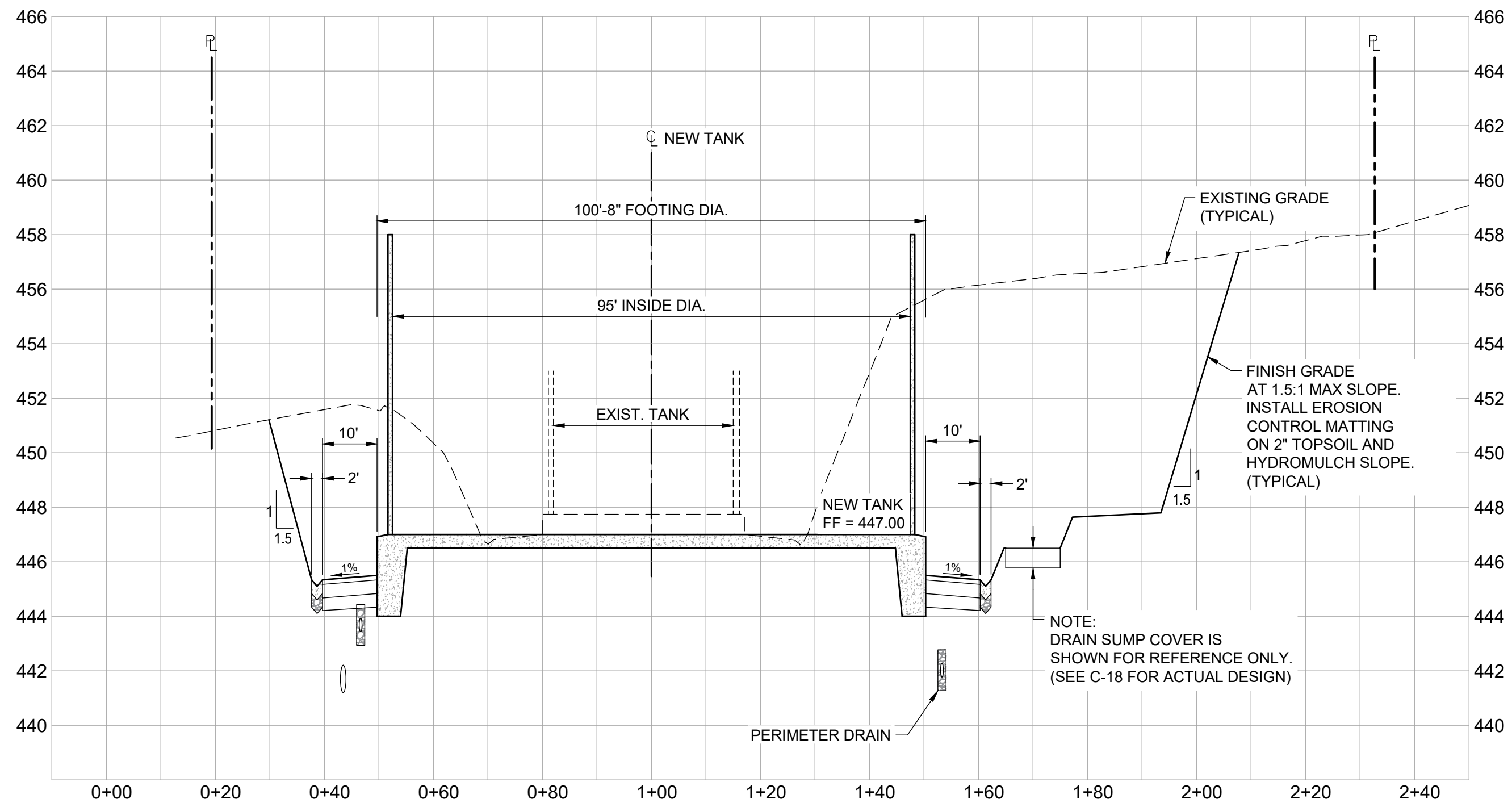
SECT B-B HORIZONTAL: 1" = 20' VERTICAL: 1" = 4'
