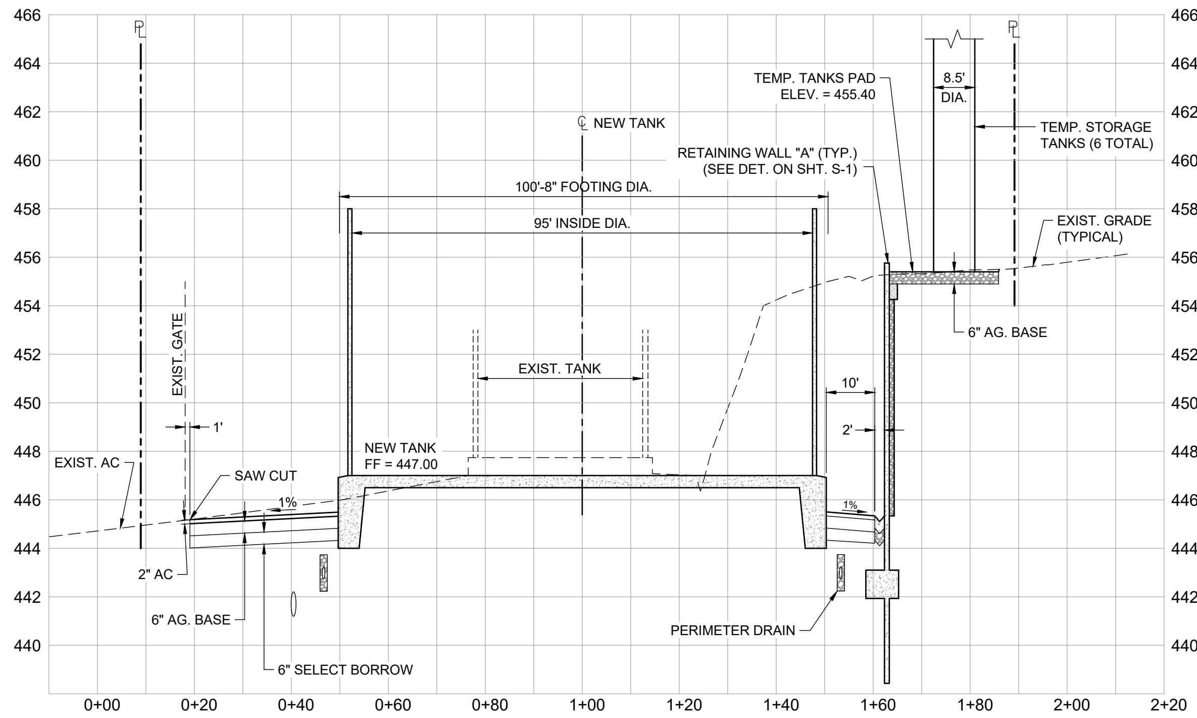
SECT A-A HORIZONTAL: 1" = 20' VERTICAL: 1" = 4'
