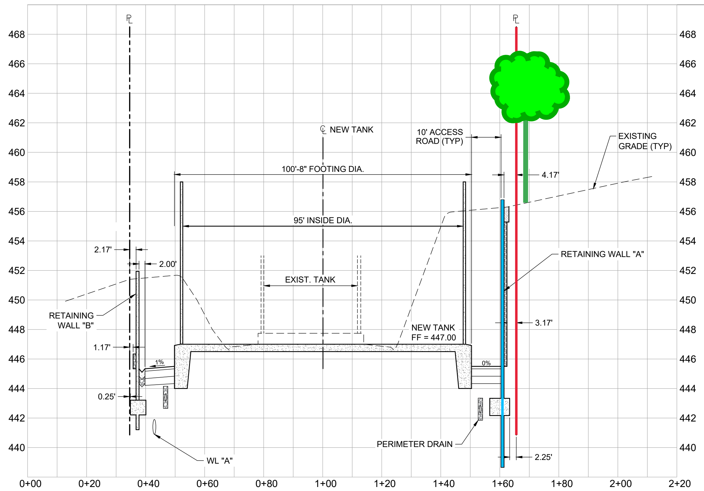
SECT C-C HORIZONTAL: 1" = 20' VERTICAL: 1" = 4'
